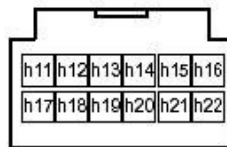
J201 (TH12) TEL/NAVI connector
